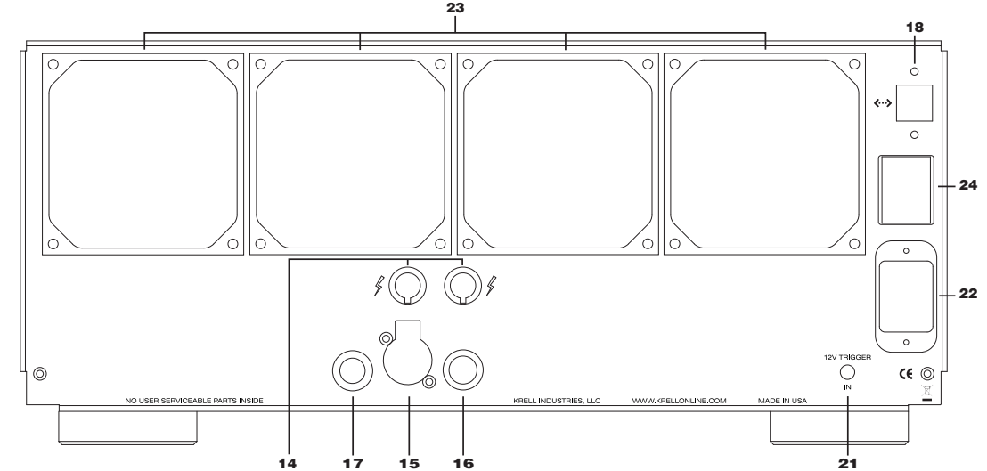
Figure 3 The iBias Back Panel - Solo 575 shown
